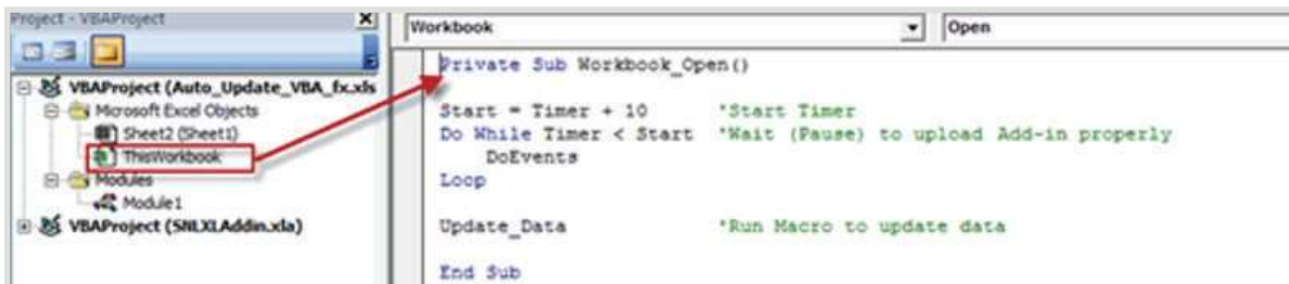
Figure 39: Adding macro to open workbook
