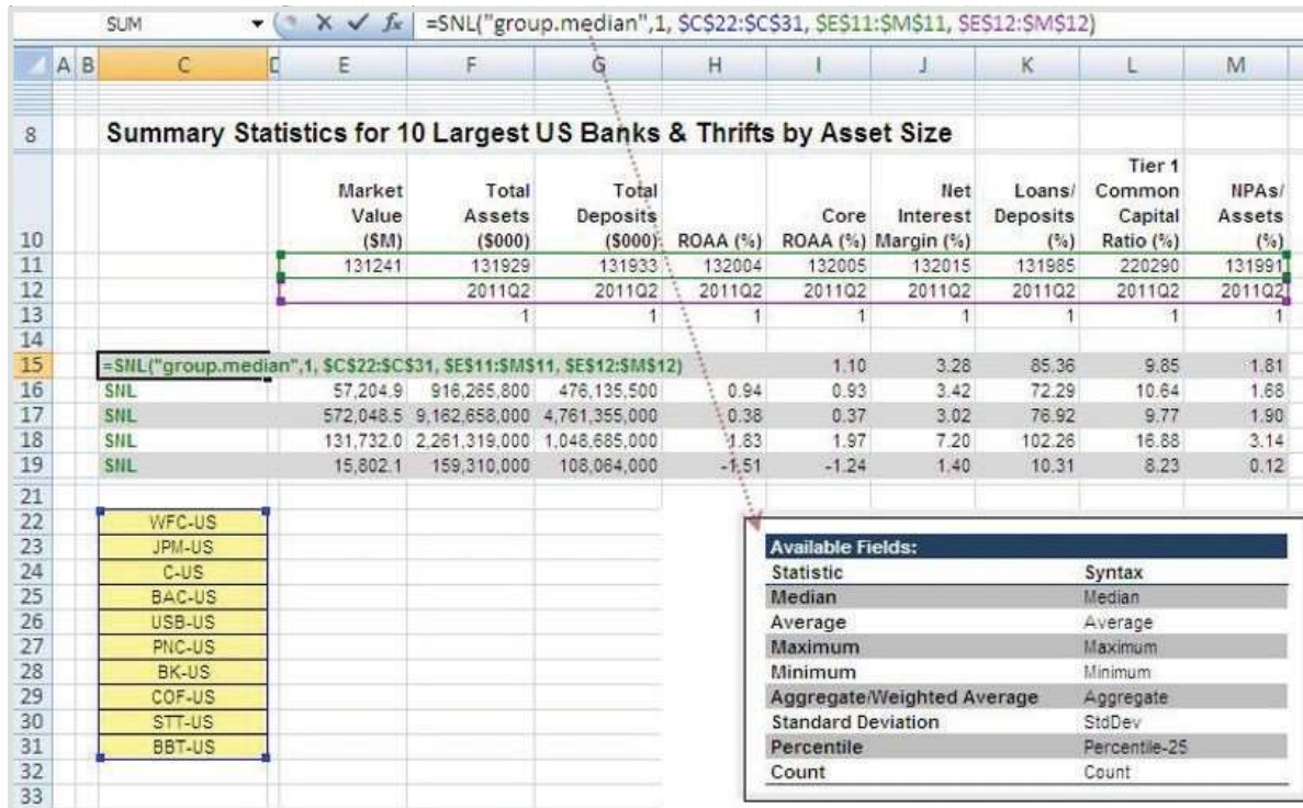
Figure 25: SNL Group function basic example
