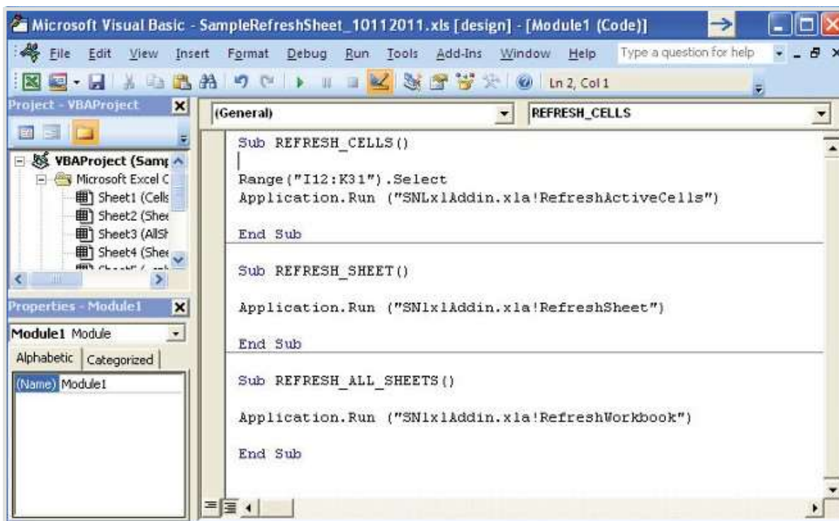
Figure 36: Example of VBA Code
