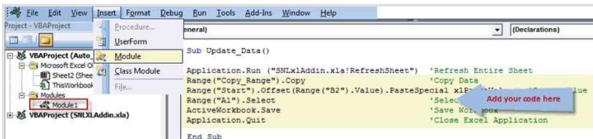
Figure 39: Adding macro to open workbook
